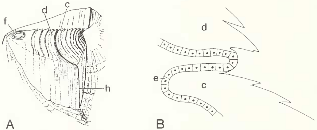
TEXT-FIG. 2. Sketches of (A) the postero-medial part of the hinge region of Clitambonites to show the orientation of the growth laminae on the deltidium and chilidium, and (B) a longitudinal section showing the envisaged relationships of the shell secreting outer epithelium to the edges of the deltidium and chilidium during growth. c - chilidium; d - deltidium; e - epithelium; f - foramen; h - hinge line.
